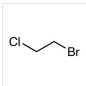
1 Bromo 2 Chloroethane
