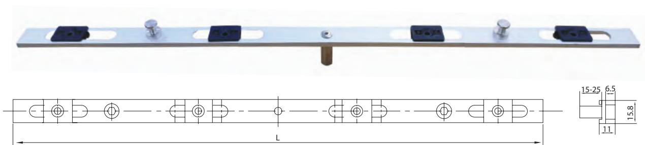
Sliding Window Espag (Non Euro Groove) L=400mm To 1600mm width 15.8mm Spindle : 25mm
