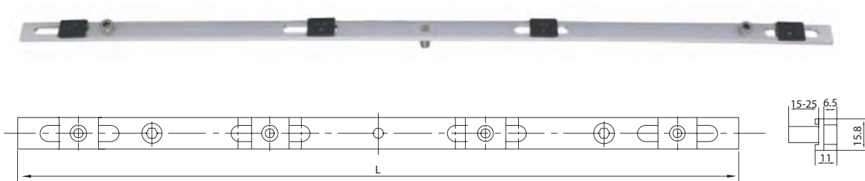
Casement Window Espag (Non Euro Groove) L=400mm To 1800mm width 15.8mm Spindle : 25mm
