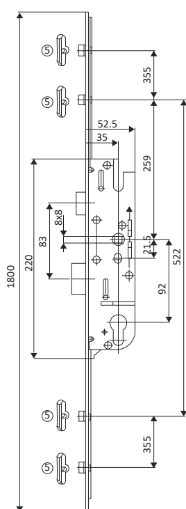
UPVC Casement Door Assembly (Auto Lock)
