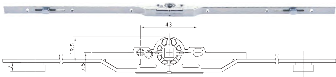
Sliding Espag Rod for 27mm/29mm/32mm/35mm & 37mm Backset : 7.5mm Length : 400mm - 2000mm Keeper : MS/SS Powder Coated
