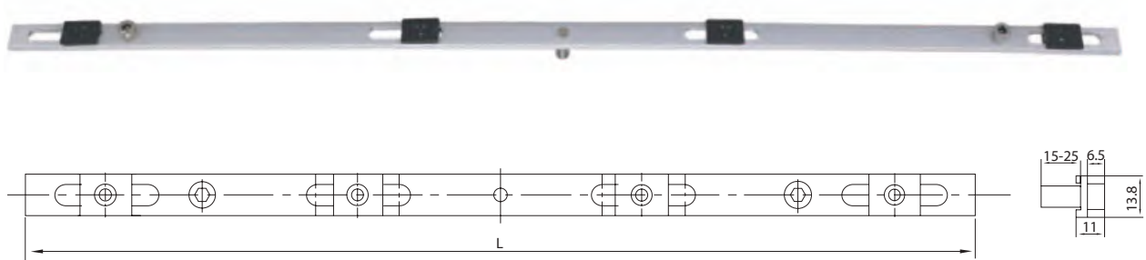
Casement Window Espag (Euro Groove) for 45mm & 52mm L=400mm To 1200mm width 13.8mm Spindle : 10mm
