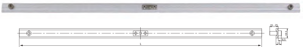
Casement Euro Groove Window Espag for Cardinal Series 50mm & 58mm L=1000mm width:19.5mm Spindle :25mm
