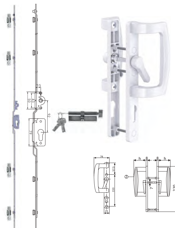
UPVC Sliding Door Lock
