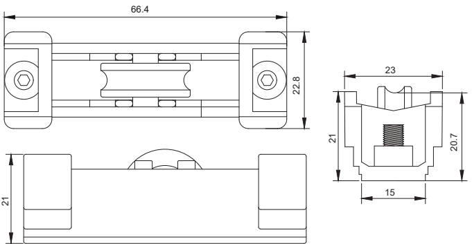
NBR-3016 (29mm Series Roller 'U' & 'V' Groove)
