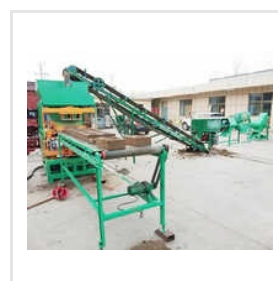
Automatic Compress Earth Block Maker
