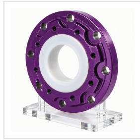
PTFE Lined Reducing Flange
