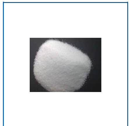
TRISODIUM PHOSPHATE ANHYDROUS
