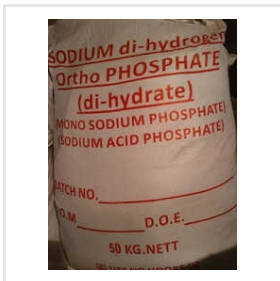
Monosodium Phosphate Dihydrate
