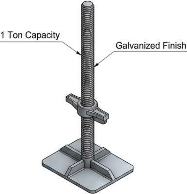
1-Ton-Adjustable-Scaffolding-Base-Jack..jpg
