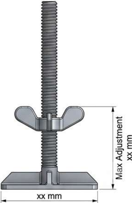
RIGHT VIEW
