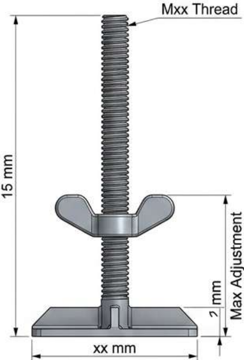
LEFT VIEW
