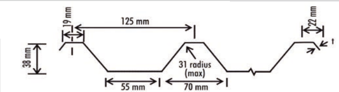
INDUSTRIAL TROUGHTED SHEET
