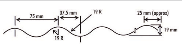
CIRCULAR CORRUGATED SHEET
