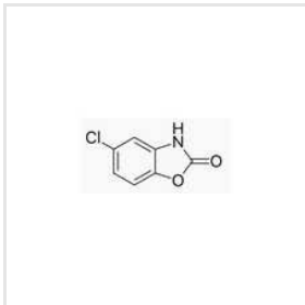
Chlorzoxazone Chemical
