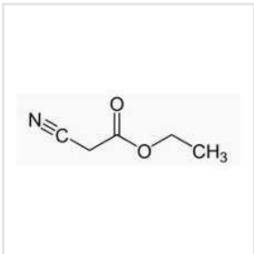
Ethyl Cyano Acetate
