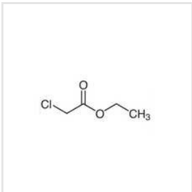
Ethyl Chloro Acetate
