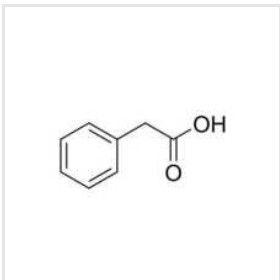
Phenyl Acetic Acid
