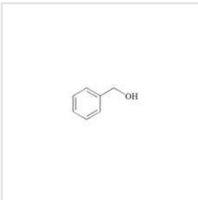
Benzyl Alcohol
