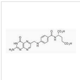
L Methyl Calcium Folate
