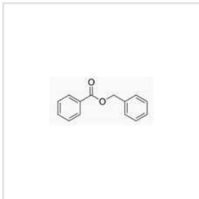
Benzyl Benzoate
