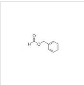
Benzyl Formate
