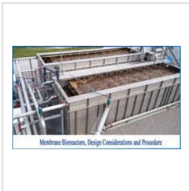
MBBR Domestic STP
