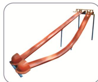
Cycloidal Path
