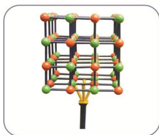
Crystal Structure
