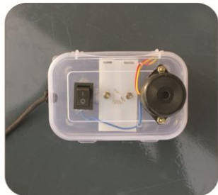
Doppler Effect
