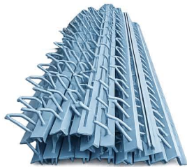
Bridge Expansion
