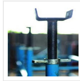
Adjustable Stirrup Heads
