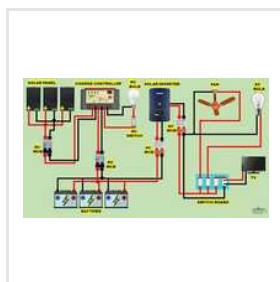
Off Grid Solar Power Plant
