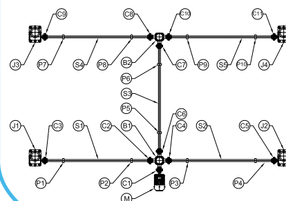
SCREW JACK WITH BEVEL GEARBOX FOR LIFTING SYSTEM
