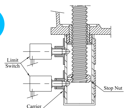
Limit Switch
