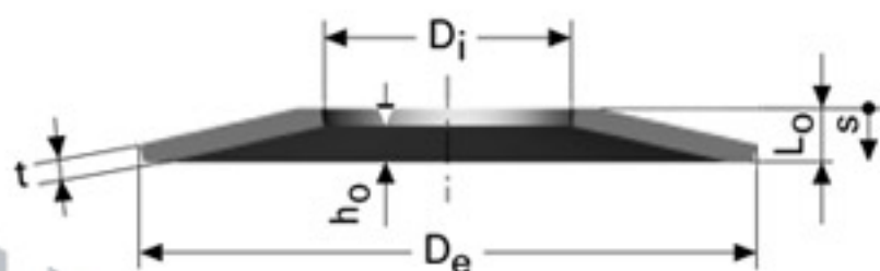
Group 3 springs
