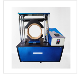
Paper Core Compression Strength Tester
