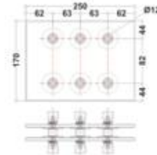
ASP-01 Splice plate Finish : Satin / Glossy Material : Stainless steel 304 grade
