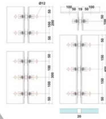
AFP-01 Fin plate Finish : Satin / Glossy Material : Stainless steel 304 grade
