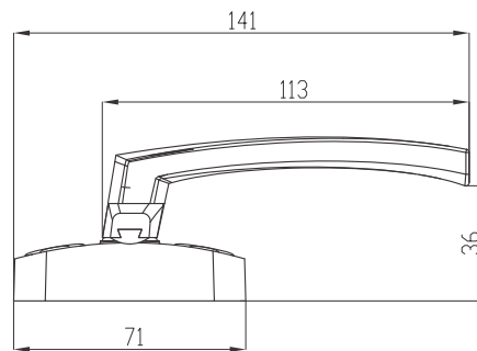
Cockspur Handle Code : PL10143L/43R
