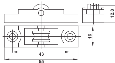
Single Roller With Groove PL50574A
