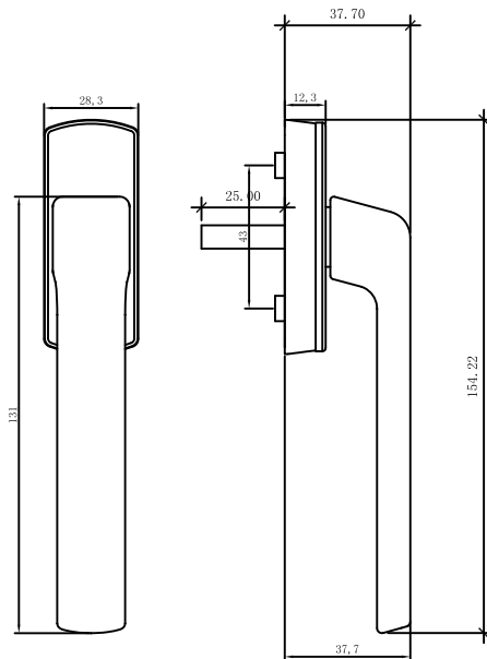
Short Neck Handle Code : PL75341
