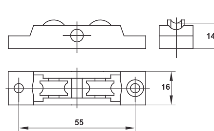
Double Roller With Groove PL50671A
