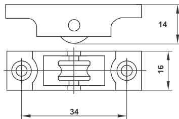
Single Roller With Groove PL50573A
