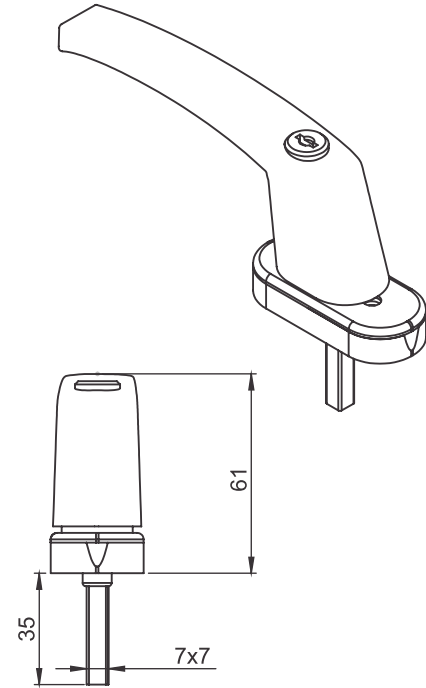
Espagnolette Handle With Key Code : PL50523
