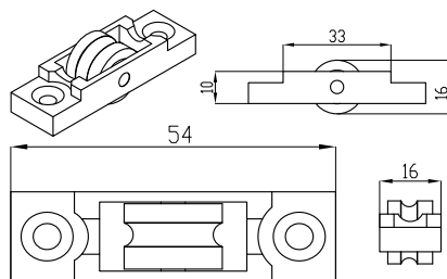
Single Roller With Groove PL50575
