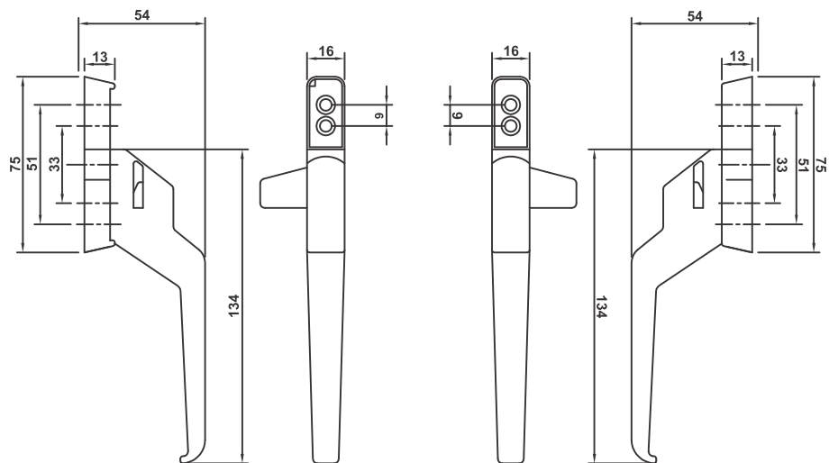
Cockspur Handle Code : PL10142L/42R
