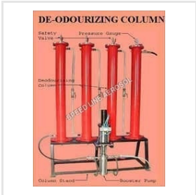
LPG De Odourizing System
