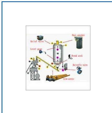
SILO ACCESSORIES
