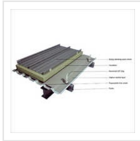
High Roof Seam Double Skin System
