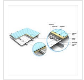
TRIMDEK Double Skin Insulated Roof System
