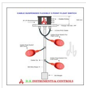
3 Point Flexible Level Switch
