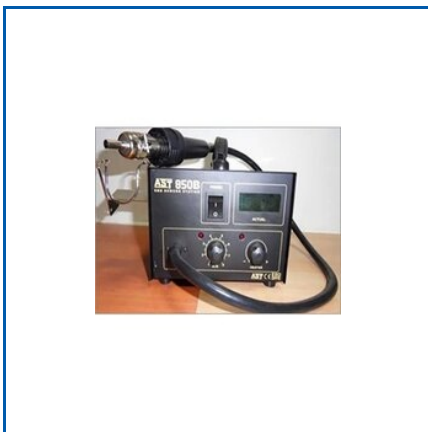
DIGITAL SMD REWORK STATION AST 850B
