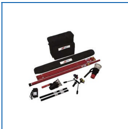
SOLO SMOKE AND CORDLESS HEAT DETECTOR TEST KIT
