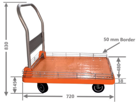
PT-150/300/500-1LB
