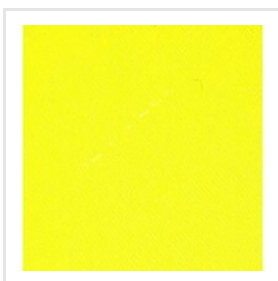
Reactive Yellow 44
