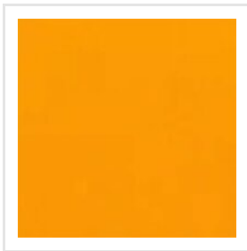
Reactive Orange 14
