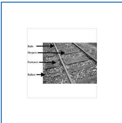
RAILWAY TRACK COMPONENTS
