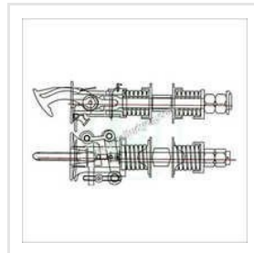
Railway Abc Coupler Assembly
