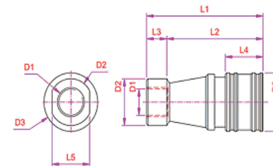
COUPLER ( BSP(F) )
