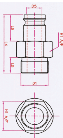
ADAPTOR ( BSP(M) )
