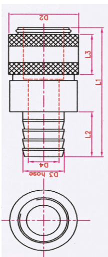
COUPLER ( HOSE )
