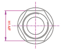
ADAPTOR ( BSP(M) )
