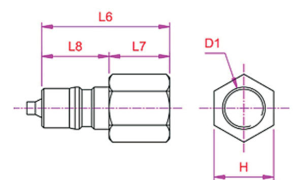
ADAPTOR ( BSP(F) )
