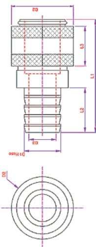
COUPLER ( HOSE )
