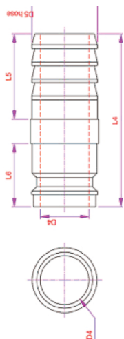
ADAPTOR (HOSE)
