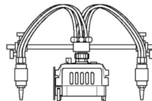
Snap Valve One-time On/Off Gas Valve Part# SNAPVALVEI : used on IK-12Max3 with 1 torch Part# SNAPVALVEII : used on IK-12Max3 with 2 torches Part# SNAPVALVEV : used on IK-12 Max3 with 300L Torch kit
