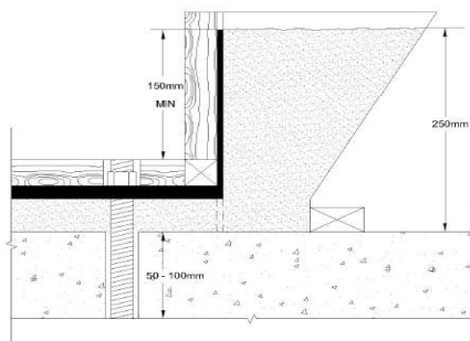
Fig.2 Typical Hopper detail
