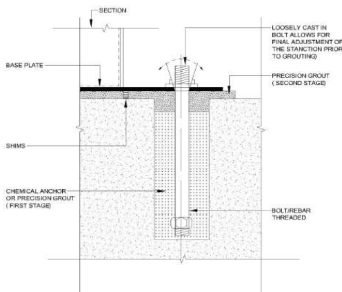
Fig.1: Typical detail of stanchion base plate
