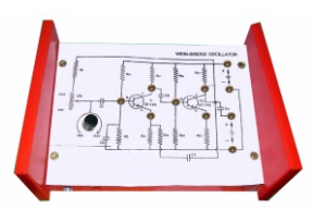
WEIN BRIDGE OSCILLATOR
