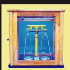
CHEMICAL BALANCE
