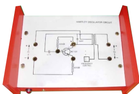
HARTLEY OSCILLATOR
