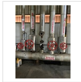
Steam Distribution Header
