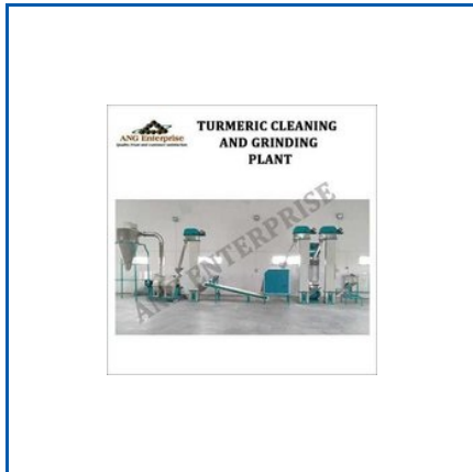
TURMERIC CLEANING AND GRINDING PLANT
