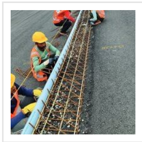
Glass Fibre Reinforced Polymer-GFRP Rebars
