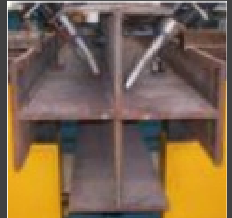
PEB H Beam Welding Line
