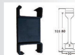
Separators
