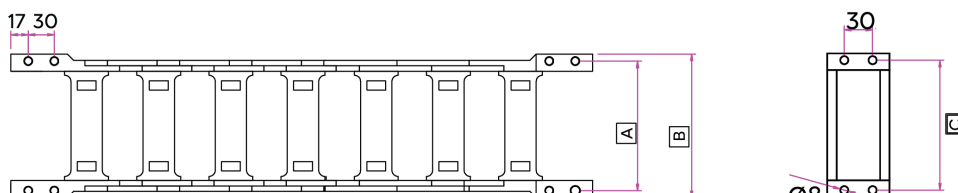
TOP VIEW
