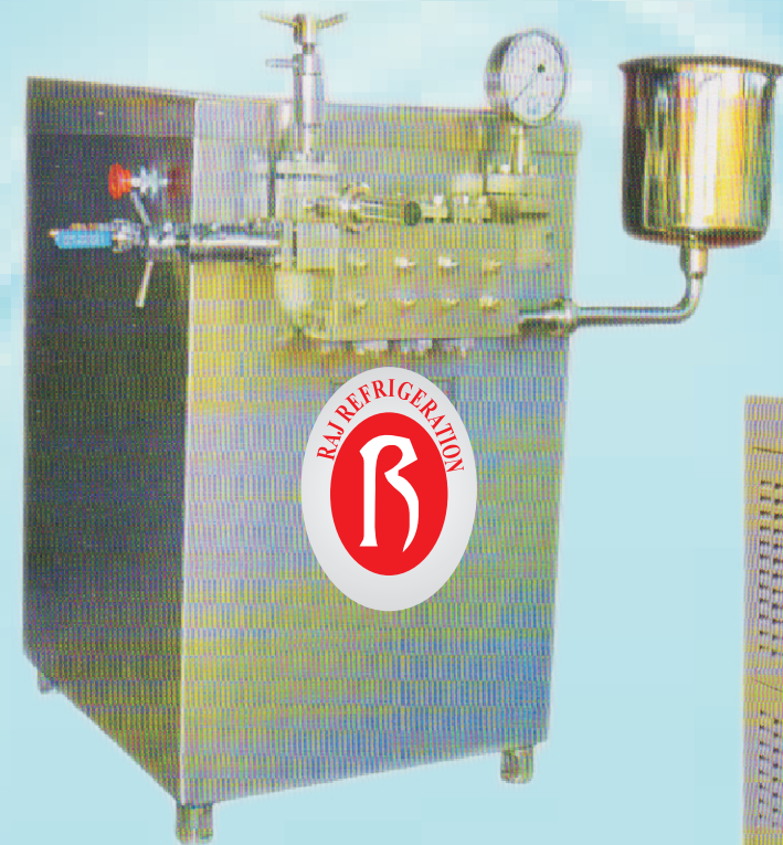
HOMOGENIZER (DOUBLE STAGE- SMALL SIZE)
