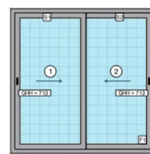
Two Track With Two Sash
