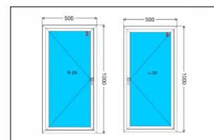
Inward Openable Left - Right
