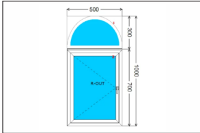
Arch Window + Openable
