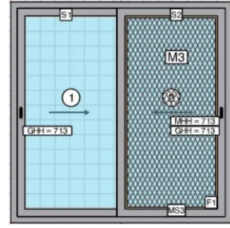
Three Track Two Sash With Mesh
