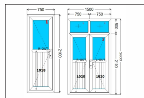
Bathroom Doors With Half Glass + Half Panel
