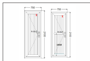
Bathroom Doors With Panel
