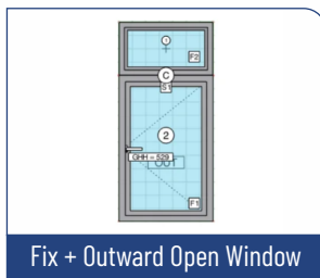
Outward Open+ Fix
