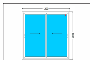
Two Track With Two Sash
