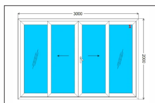
Two Track With Four Sash Side Fix + Center Sliding
