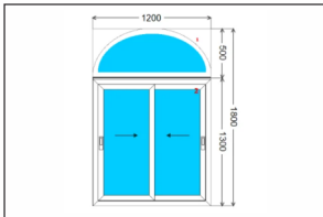
Arch Window + Sliding
