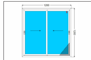
2+1 Track Two Sash + Mesh
