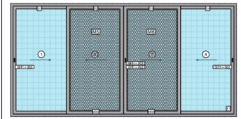
Three Track Six Sash + Mesh
