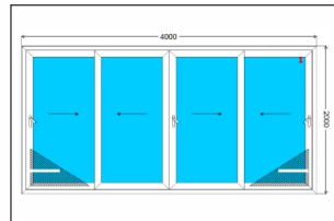
Three Track With Six Sash + Mesh
