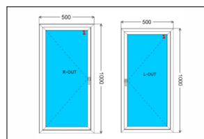
Outward Openable Left - Right
