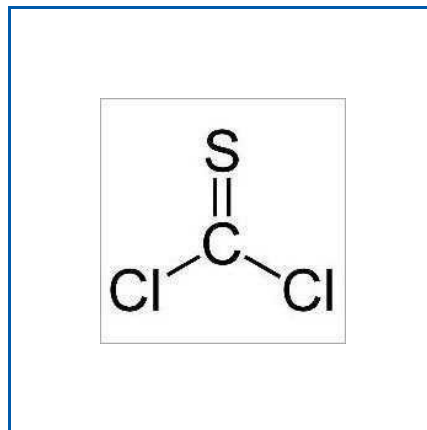
LIQUID THIOPHOSGENE
