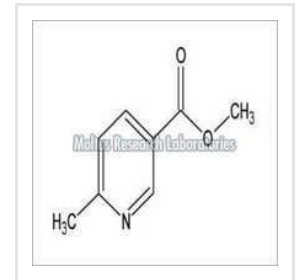
Methyl 6-Methylnicotinate
