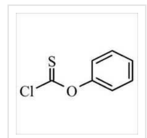
Phenyl Thiochloroformate
