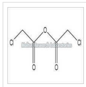
Chloroacetic Anhydride
