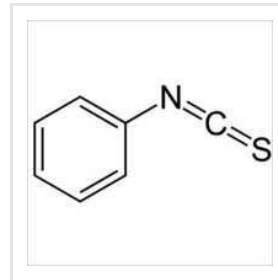
Phenyl Isothiocyanate
