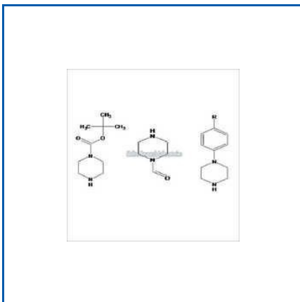
PIPERAZINE DERIVATIVES
