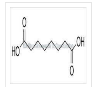
Suberic Acid
