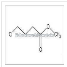
Methyl 4-Chlorobutyrate
