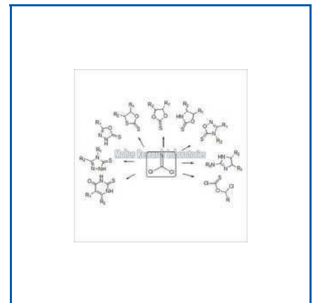
THIOPHOSGENE
