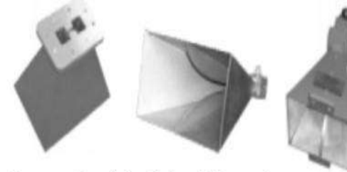
Octave Double Ridged Horn Antenna
