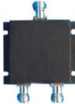
2 Way Power Splitter 150~1000 MHz
