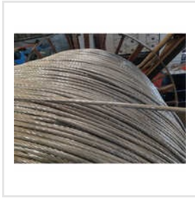
ACSR Weasel 30 SQ MM Conductor
