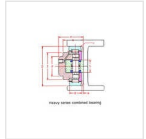
Heavy Series Combined Bearing
