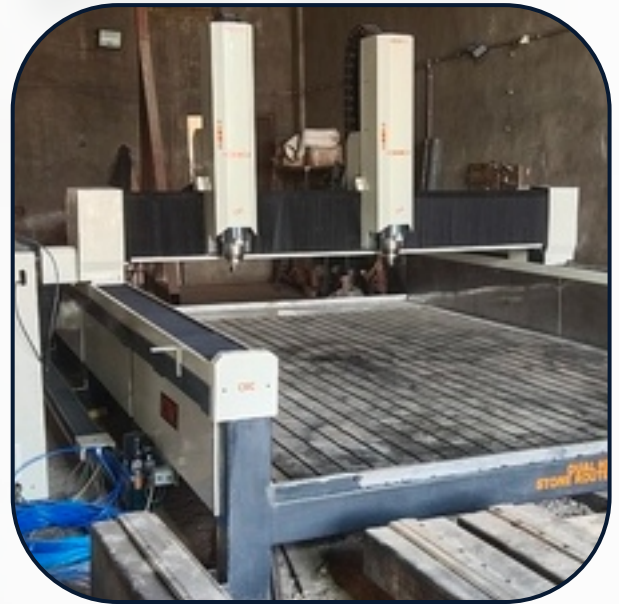
Double Head Cnc Router Machine
