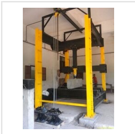
Structural Loading Frame
