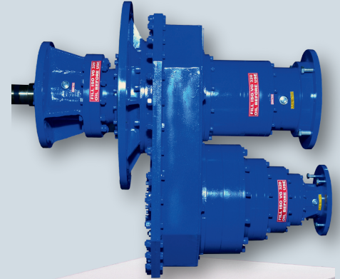
Dual Input Flange Type Planetary Gearbox
