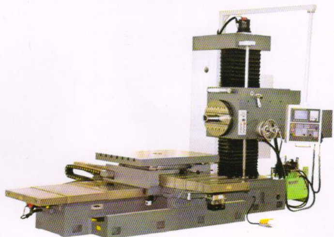
Heavy Duty Conventional & Cnc Boring Machine
