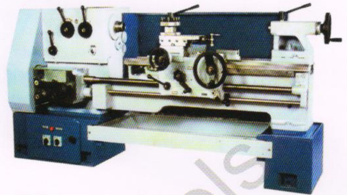
All Gear Lathe Machine
