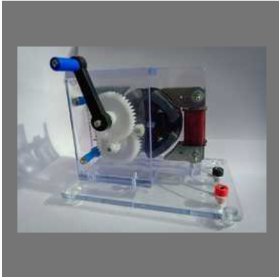
Hand Cranked AC/DC Generator Demonstration Kit
