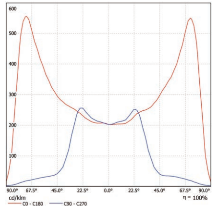
L709-RXT Distribution Curve
