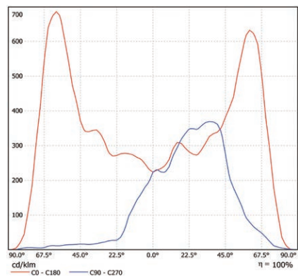
L712-AB Distribution Curve
