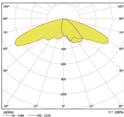
L712-AB Distribution Curve
