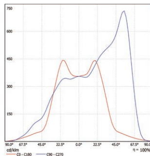
L735-AB Distribution Curve
