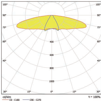
L709-RXT Distribution Curve
