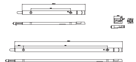
ARH 21 Shoot Bolt available in Black, White. Size: 250 mm and 425 mm.
