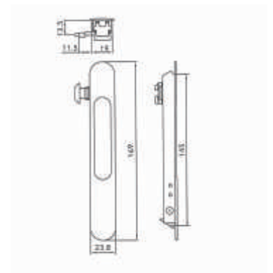
ARH 19 Concealed Lock packing : 100pcs/Box available in Black, White and Champagne Gold
