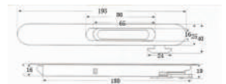
ARH 20 Dual Lock packing : 100pcs/Box available in Black, White.
