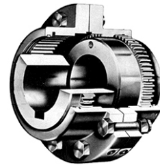
GEAR COUPLING
